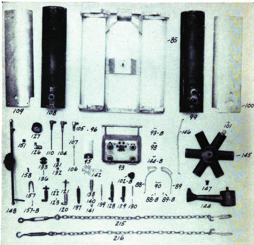
① FIGURE 38.—Gasoline fire unit parts and tools.
